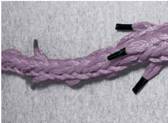
Moran 5/4/3 Tuck Splice close up of tails and tuck area below eye splice
