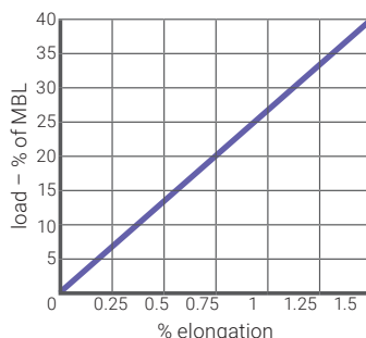
Vectran® 12-Strand & 12x12 Elongation (%)
