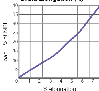
Polyester Double Braid Elongation (%)
