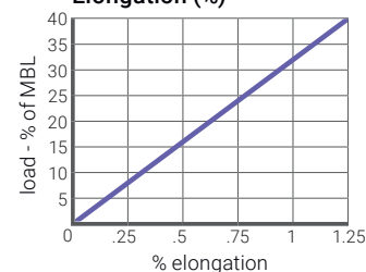
Plasma® HiCo 12-Strand Elongation (%)
