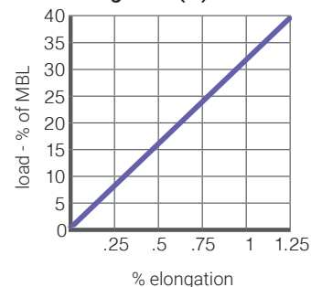
Toro® 12-Strand Elongation (%)
